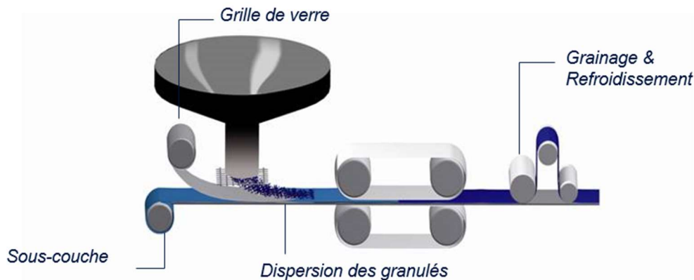
Figure 2 : Process de Pressage
