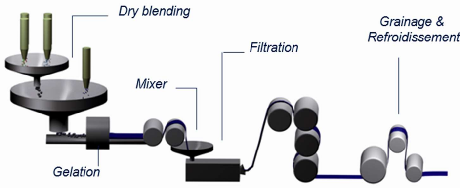
Figure 1 : Process de Calandrage
